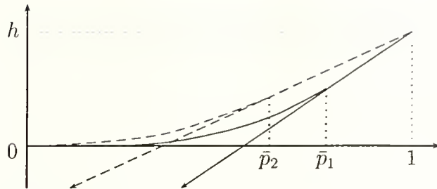
Figure 3: A Payoff Shift in the R&D Model. When the (unplotted) bad build payoff \ell rises, so does the value function, and intensity levels (inside the now left-shifted interval (\underline{p}, \bar{p}) ).
