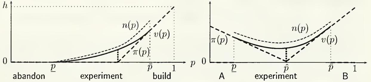
Figure 2: Value Function and Experimentation Demand. Overusing the vertical axis, we depict both the static payoff function \pi (thick dashed line) and dynamic value function v (solid line), strictly convex in the experimentation domain \mathcal{E} = (\underline{p}, \bar{p}) , and the intensity level n (thin dashed line). The demand is increasing in v . The R&D model is illustrated on the left, and a more general decision model (no null action) on the right. The option value of experimentation — the vertical distance between the static and dynamic values — is maximized at the \pi kink \hat{p} .
